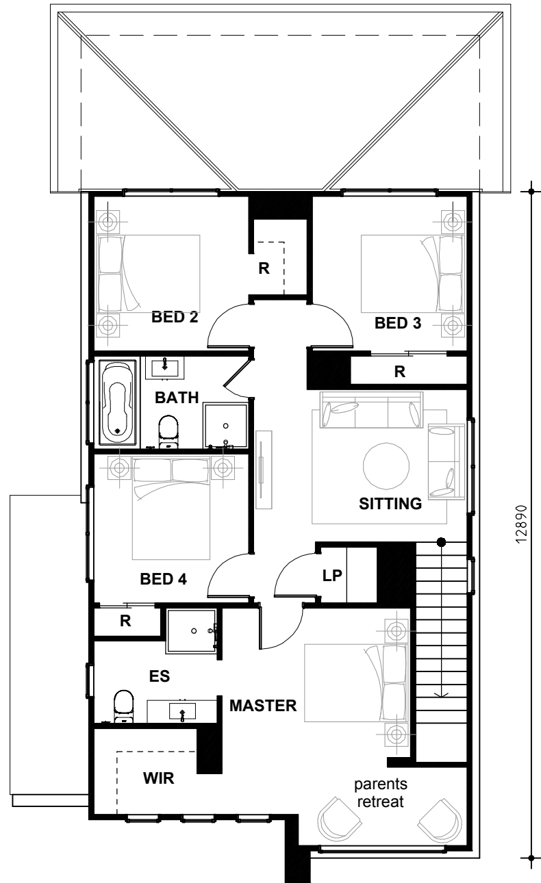
7550 FIRST FLOOR PLAN
